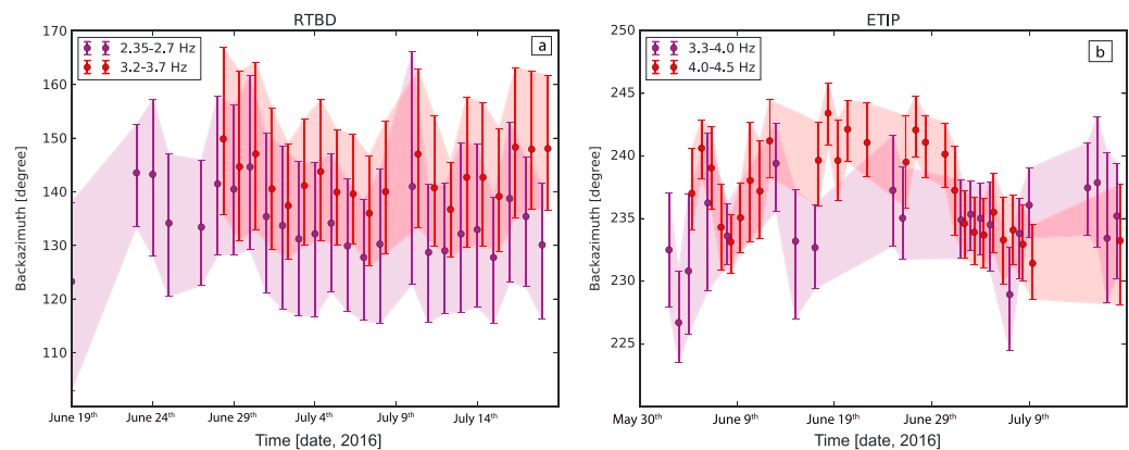
Figure 5. Time series of back azimuth estimations for (a) RTBD and (b) ETIP. Colors represent different frequency band of Rayleigh wave glaciohydraulic tremor. The dots represent the median back azimuth for a given day within a frequency band, while the error bars represent the 25 th and 75 th percentiles of estimates. The envelopes trace the 25 th and 75 th percentiles.
