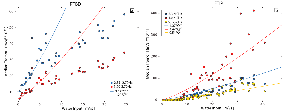
Figure 9. Relationship between water input and the median tremor power at (a) RTBD and (b) ETIP. Each point represents 1 day. The lines represent the P_w \propto Q^{5/4} relationship that is mentioned in Gimbert et al. (2016) with each line having a different scaling factor that is specified in the legend.
